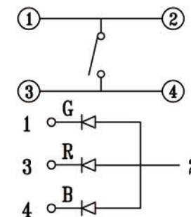
SCHEMATIC
