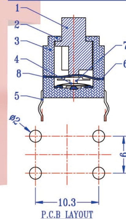
SCHEMATIC
